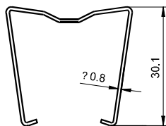
14FF-H2 (Metallic retainer)
